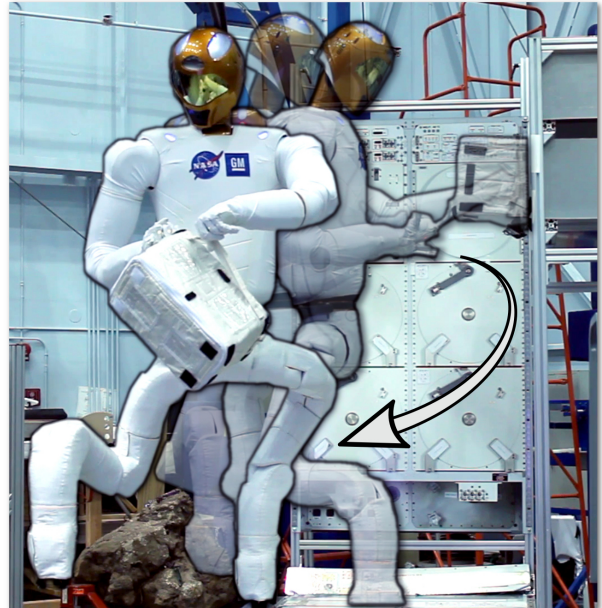
Fig. 1. R2 executing the CTB retrieval scenario. R2 has to respect many different constraints when planning motions along the course of the operation. For example, when holding the CTB with both hands, there is a constraint imposed on the hands as to not drop the CTB. The system allows consideration of constraints such as the example given and provides means for the operator to easily specify novel ones without leaving the high-level interface. There are four stills superimposed in this image, from back to front: R2 approaching the cargo rack, R2 unbuckling the restraint holding the CTB, R2 grabbing the CTB with both hands, and the final image of R2 bimanually manipulating the CTB.
