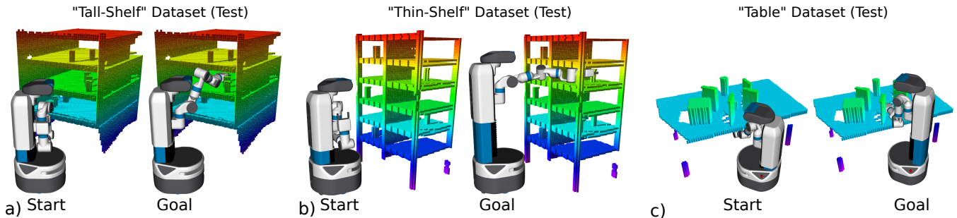
Fig. 5. The three datasets used to test the evaluated methods. Different problems are generated similarly to Fig. 4. a) An example environment from the “Tall-Shelf” dataset. The “Tall-Shelf” is created by stacking the “Small-Shelf” three times. b) An example environment from the “Thin-Shelf” dataset. This is also a bookcase like “Small-Shelf” and “Tall-Shelf”, but the shelves are shorter and there is a divider, making it a much more challenging problem. c) An example environment from the “Table” dataset, which includes a table with several objects and is very different from the other datasets.
