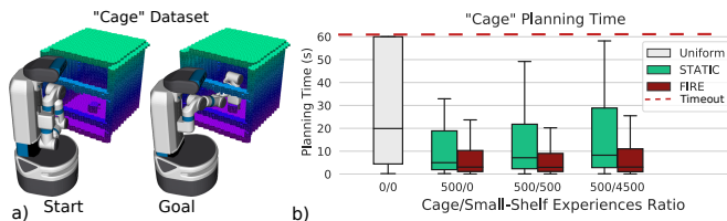
Fig. 7. a) An example problem from the “Cage” dataset. b) Planning time for 100 test examples from the “Cage” dataset using the RRTC-TUNED planner. The timeout was set to 60 seconds. The x-axis shows the number of experiences that exist in \mathcal{DB} from “Small-Shelf” and from “Cage”. Note that “Small-Shelf” and “Cage” have very different solution paths. In other words, the experiences from “Small-Shelf” do not transfer to “Cage”.
